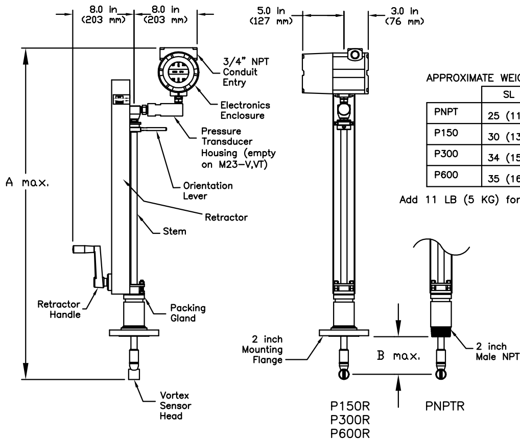
MODEL M23 in (mm) WITH PERMANENT RETRACTOR
